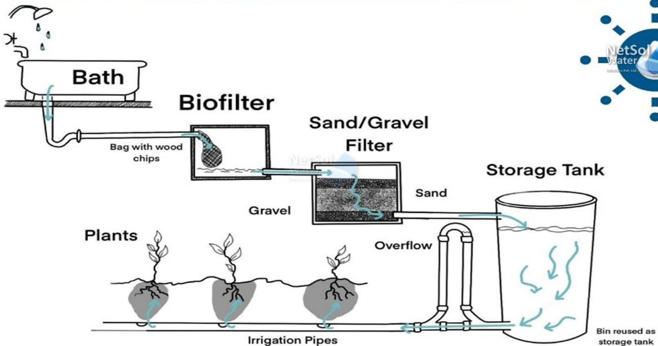
Working of a Grey Water System
